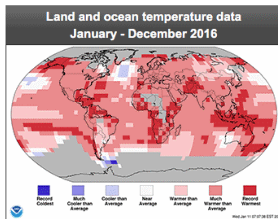
[+] This January-to-December map of temperature anomalies shows that higher-than-average temperatures occurred across the vast majority of the globe during 2016, combining to bring overall record warmth for 2016. Climate change skeptics have called these data into question. Graphic courtesy of the National Oceanic and Atmospheric Administration.
